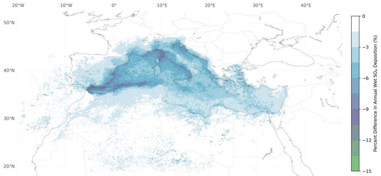
Figure 18: Percent decrease in annual wet sulphate deposition between MARPOL VI and Med ECA
