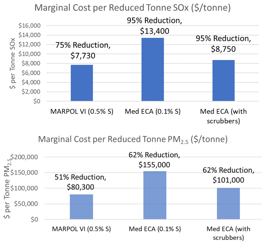
Figure 29. Control cost-effectiveness of SOx and PM2.5 reductions based on prices in this study
