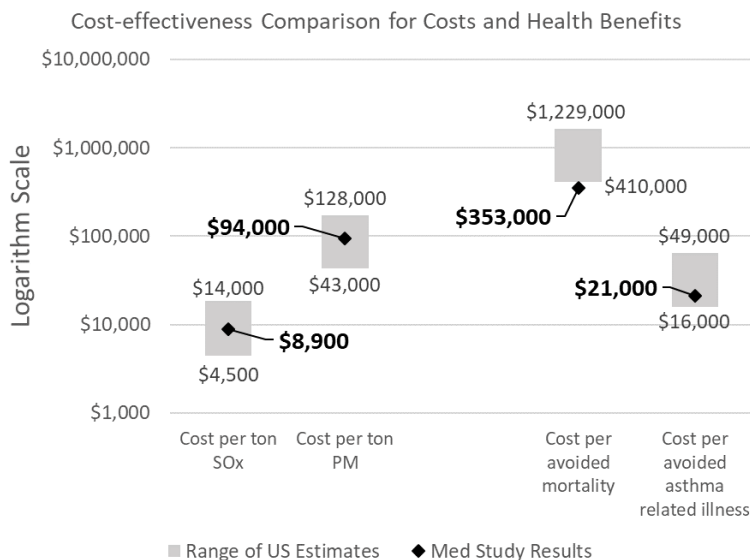
Figure 32. Summary Comparison of cost-effectiveness metrics for this study (combining MARPO VI and Med ECA measures) with U.S. SOx and PM data from the Proposal to Designate an Emission Control Area for North America.
