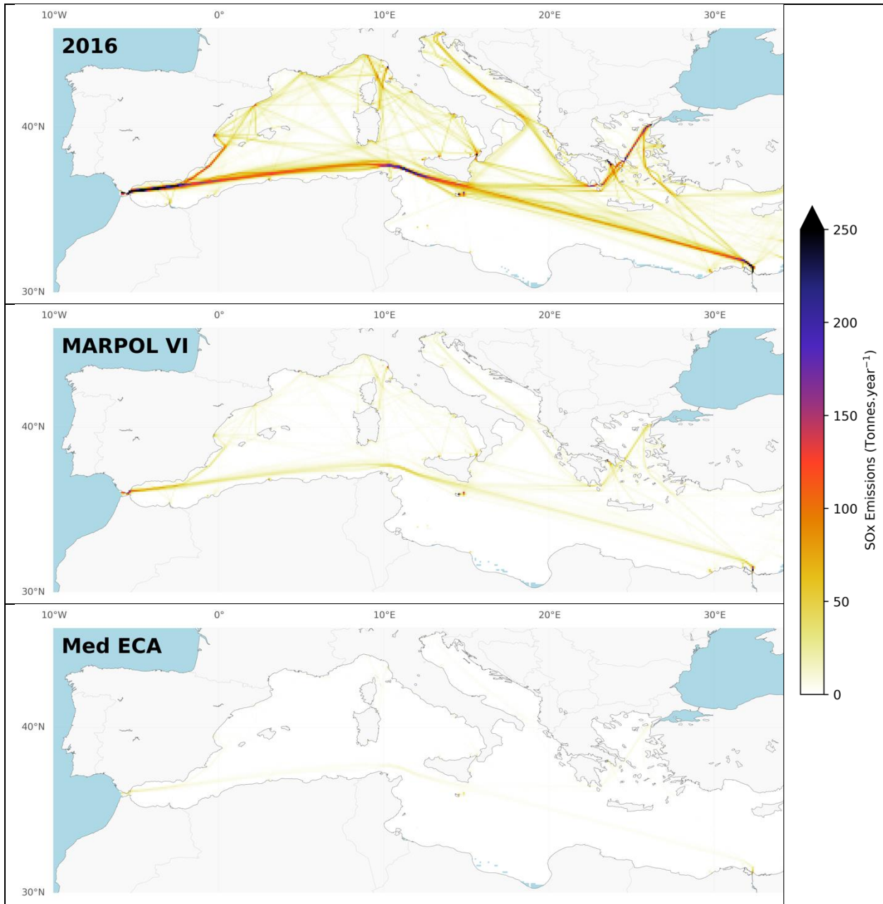
Figure 10: SOx emissions under 2016 baseline, 2020 MARPOL VI, and 2020 Med ECA scenarios
