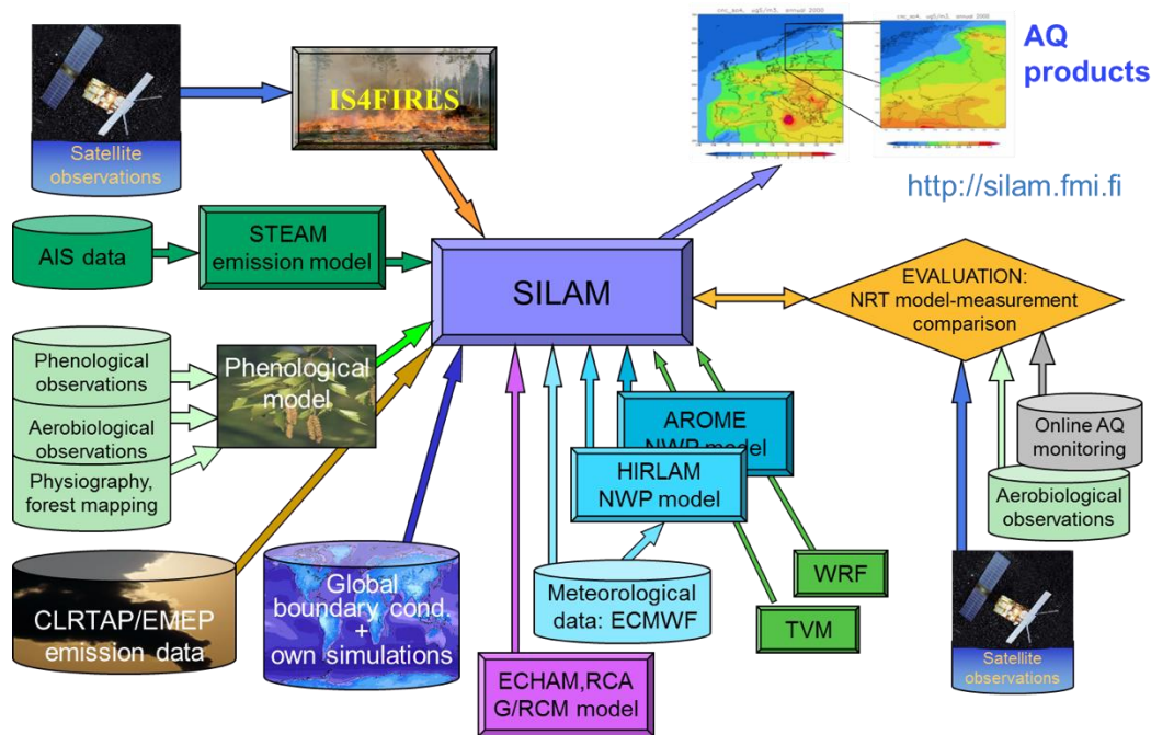
Figure 33: Schematic representation of the STEAM/SILAM system for air quality research problems.
