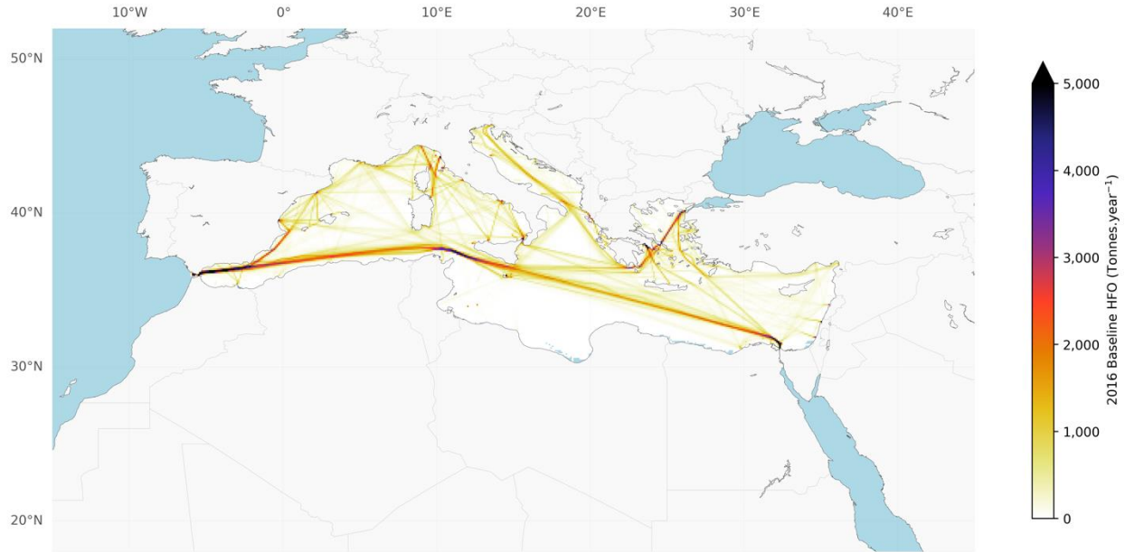
Figure 9: Baseline 2016 HFO fuel use
