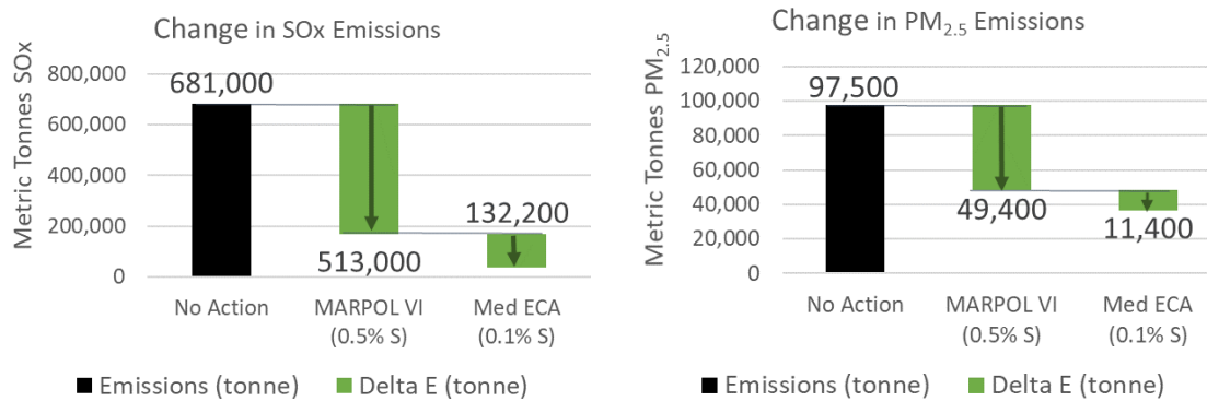
Figure 3. Change in SOx and PM 2.5 emissions under different Mediterranean regulatory scenarios
