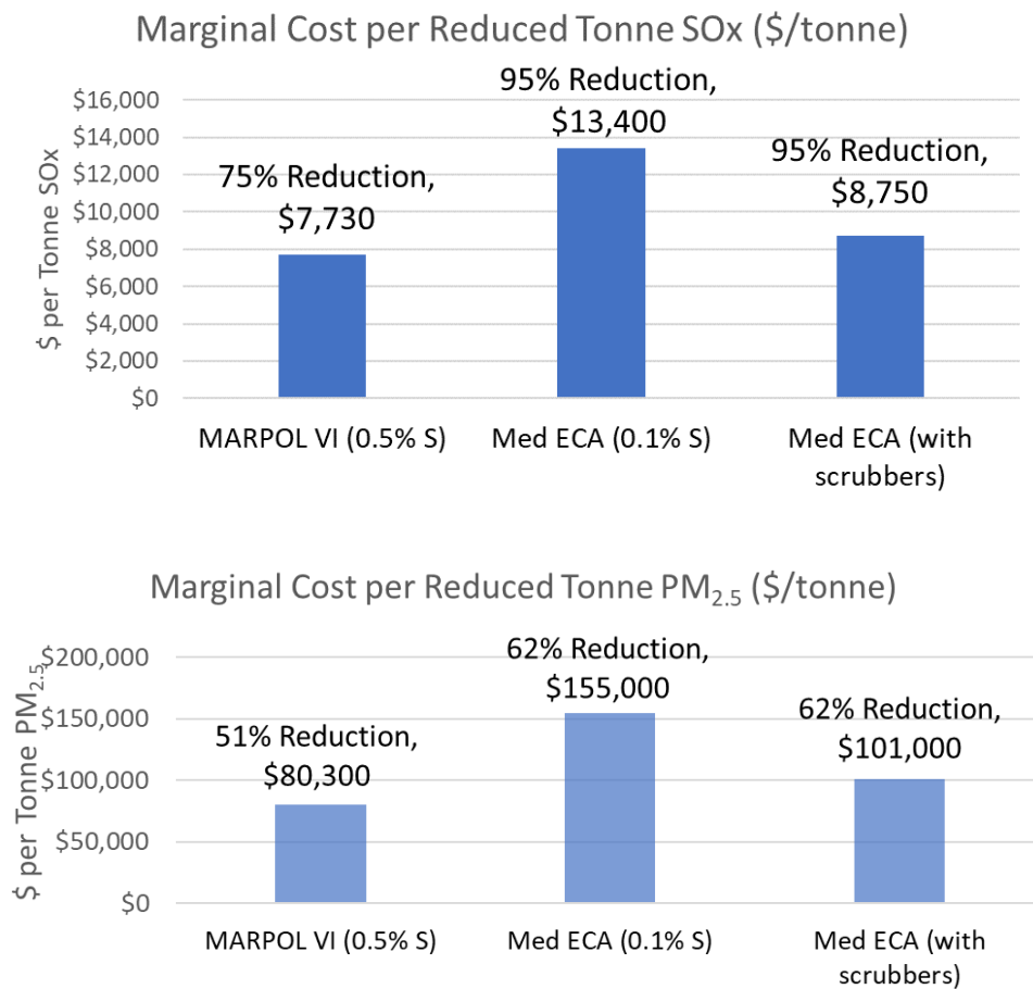
Figure 5. Control cost-effectiveness of SOx and PM2.5 reductions based on prices in this study
