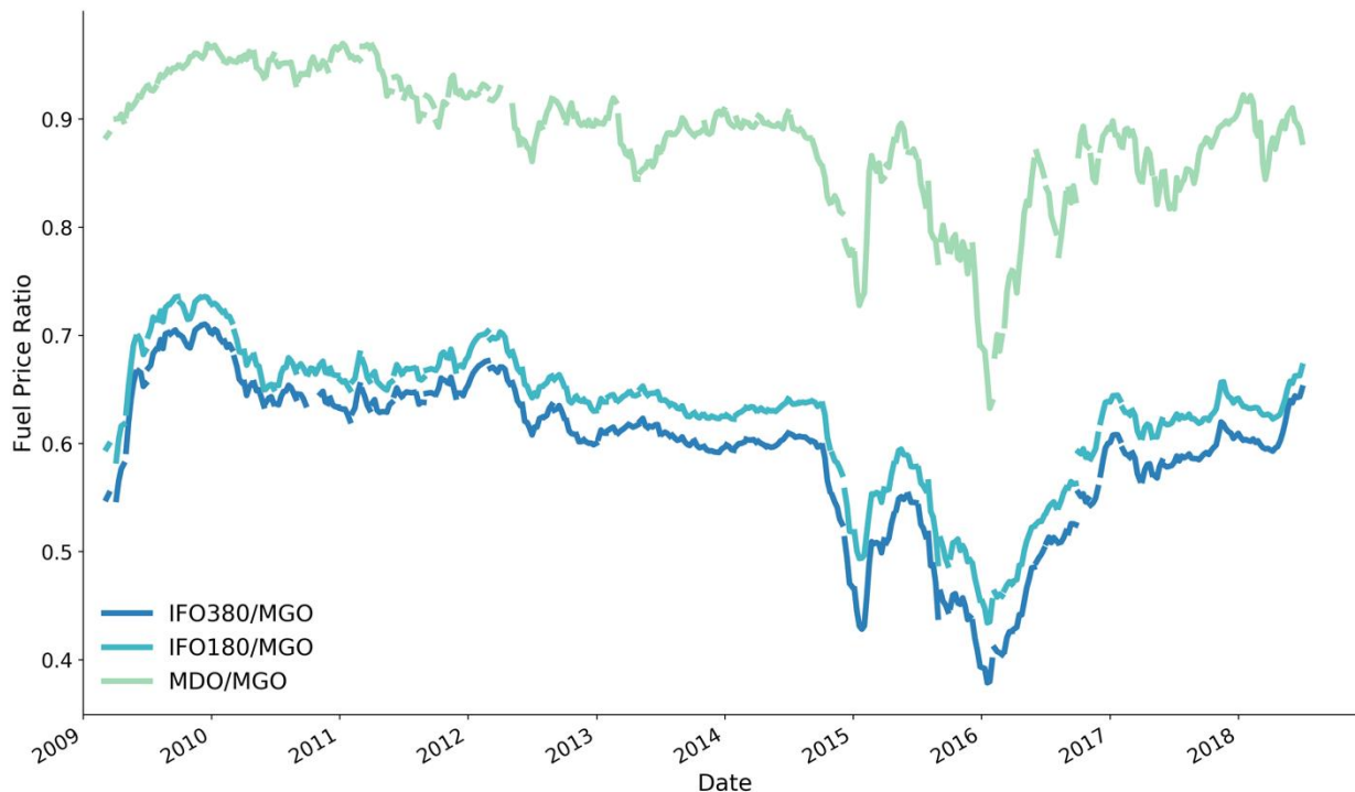
Figure 35: Price ratio of MGO to IFO380, IFO180, and MDO
