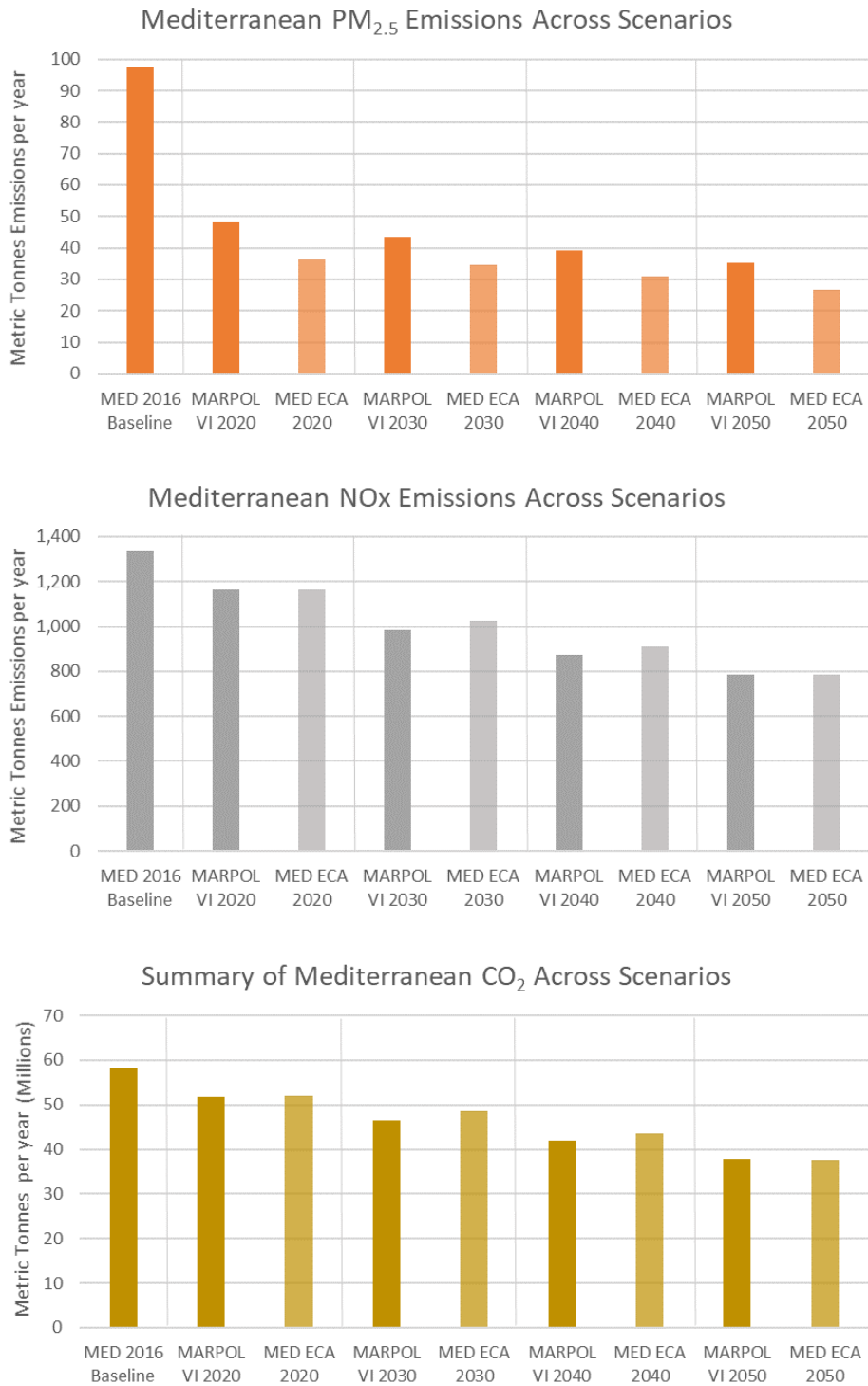
Figure 15. Multi-year estimates for PM 2.5 , NO x , and CO 2 from shipping in Mediterranean Sea Area
