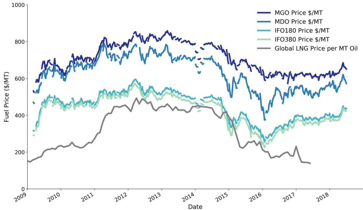
Figure 34: Bunker prices for marine bunker fuels from 2009 to 2018, resampled to mean weekly prices, in 2015 USD/MT.
