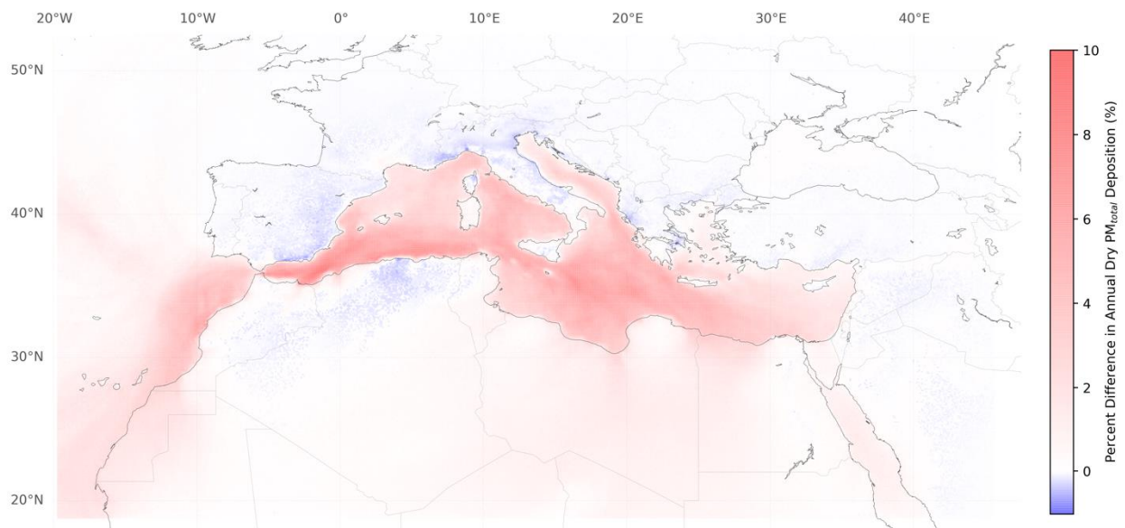
Figure 24: Percent change in annual dry PM_{Total} deposition between MARPOL VI and Med ECA
