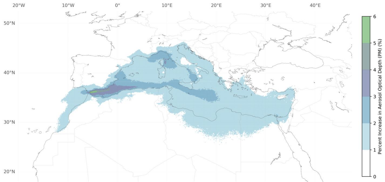
Figure 25: Percent Change in aerosol optical depth (PM species) between MARPOL VI and Med ECA
