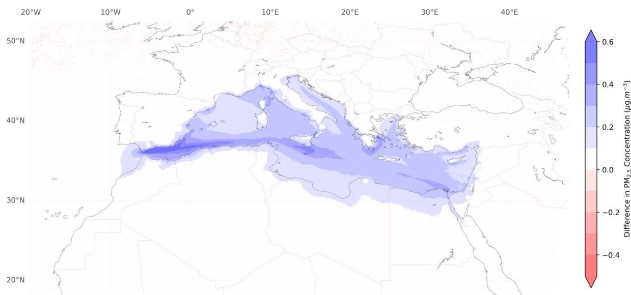
Figure 16: Difference in PM_{2.5} concentration between MARPOL VI and Med ECA scenarios
